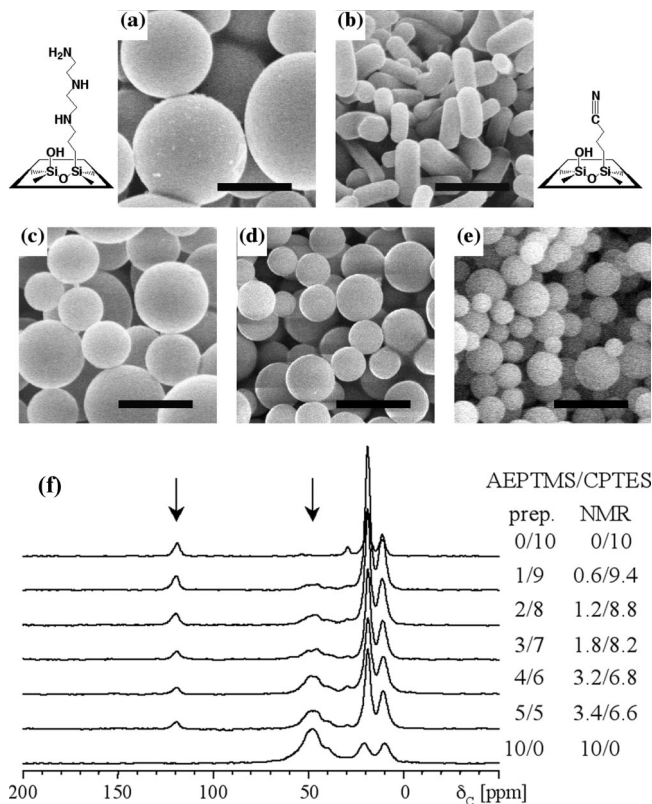
FIGURE 2. FESEM images of (a) N -(2-aminoethyl)-3-aminopropyl-MSN (AEP-MSN), (b) 3-cyanopropyl-MSN (CP-MSN), (c) 5:1 AEP/CP-MP, (d) 3:1 AEP/CP-MP, and (e) 1:1 AEP/CP-MP. Scale bar = 1 \mu m. (f) Cross-polarization magic-angle spinning ( 13 CPMAS) spectra of AEP/CP-MPs. Arrows show the resonances that are unique for each species and thus were used for quantitative analysis. The numbers represent the molar ratio between two components used for preparation and obtained from analysis of NMR spectra. Reproduced with permission from ref 14. Copyright 2003, Royal Society of Chemistry.
